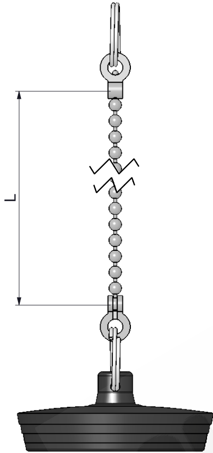
Plug with chain Tappo catena
